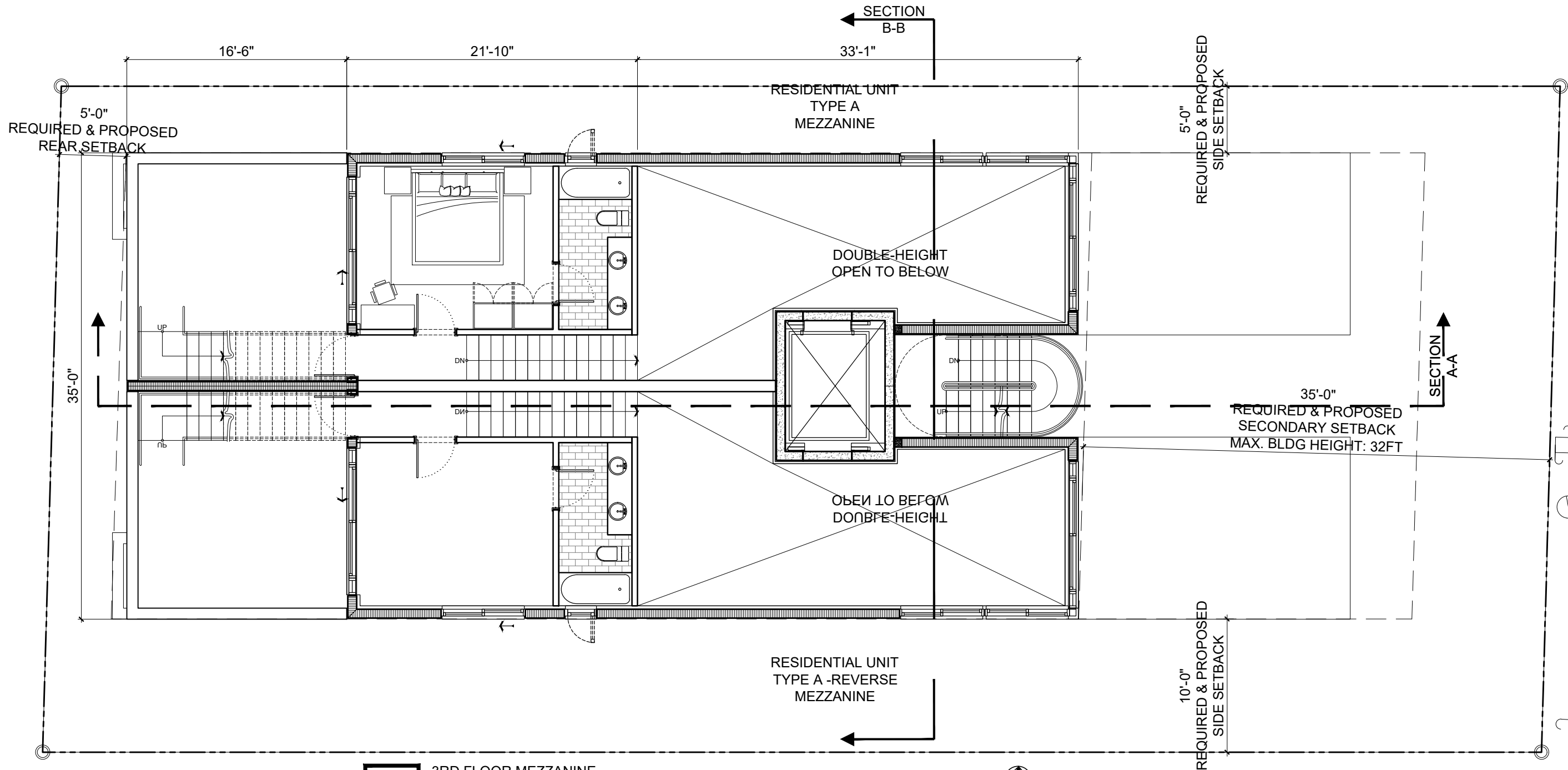
1 3RD FLOOR MEZZANINE SCALE: 1/8" = 1'-0"
